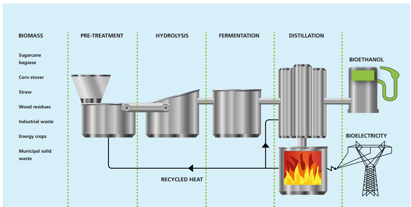
Fig. 8. General process flow for second-generation ethanol production.
