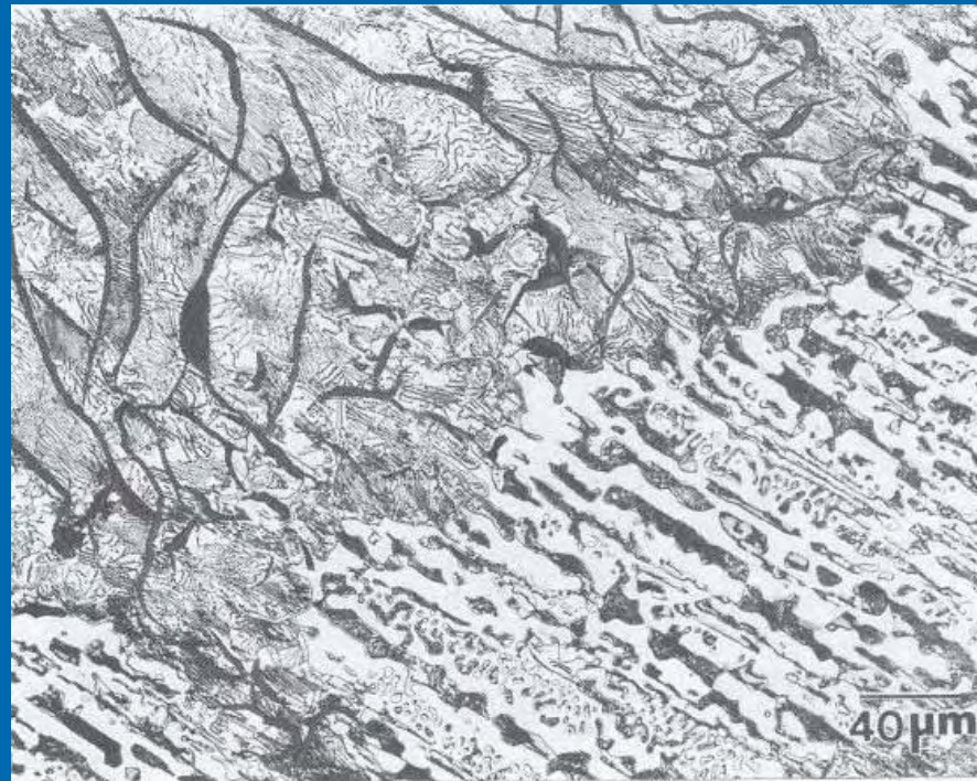
Fig. 2.50 Mottled pearlitic cast iron. Gray iron at upper left and white iron at lower right of photo. 4% picral etch. 250×
