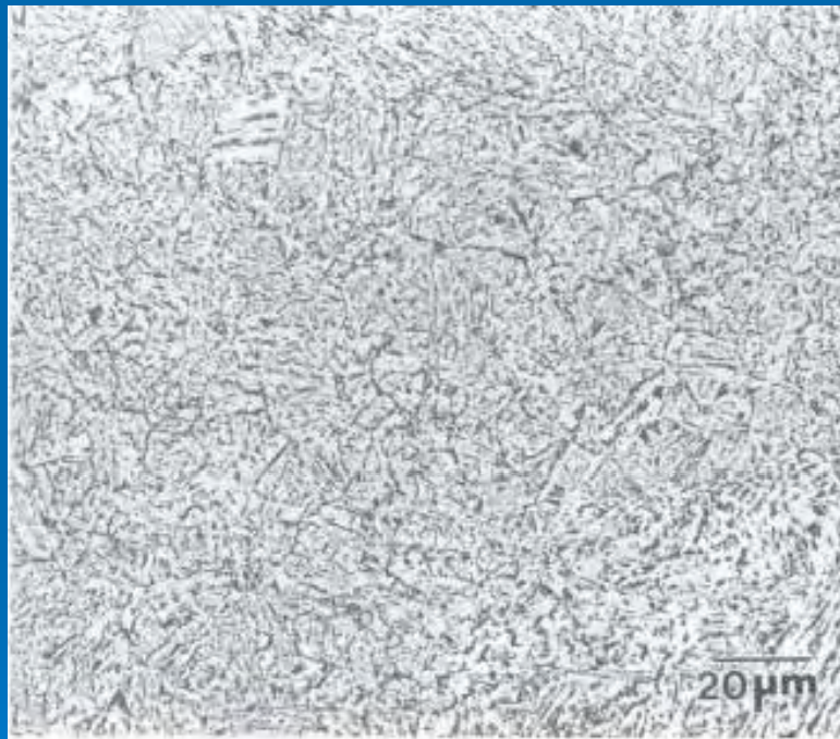
Fig. 2.33 Upper bainite in an AISI/SAE 8720 steel isothermally transformed at 425 °C (797 °F) for 90 s. 4% picral etch. 500×
