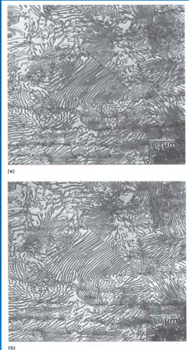
Fig. 5.24 Micrographs of an AISI/SAE 1080 steel showing the same field of pearlite taken with (a) a dry objective of NA = 0.90 and (b) and oil-immersion objective of NA = 1.30 . Note the improved resolution in the micrograph taken with the oil-immersion objective. 4% picral etch. 1300\times . Courtesy of S. Lawrence, Bethlehem Steel Corporation
