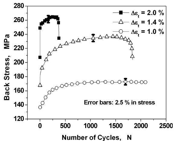
Fig. 4. Variation of the back stress with cycles in Zircaloy-4.
