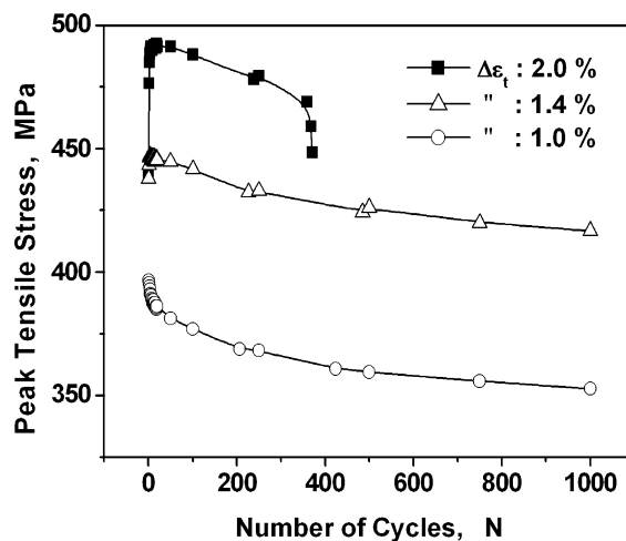
Fig. 1. Cyclic softening observed in Zircaloy-4 at three different total strain ranges.
