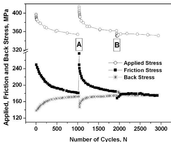
Fig. 5. Applied, friction and back stresses during a test with interruptions. Point A, test interruption with thermal annealing one hour at 573 K. Point B, test interruption with thermal annealing one hour at 473 K (see text).
