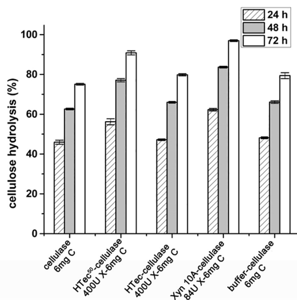
Fig. 1. The effect of different pretreatment methods of 1st stage on cellulose yield and the total enzyme dosage (mg/g cellulose) used in the hydrolysis of Kraft pulp (KP) at 2%. Cellulose yield was monitored after 24 h, 48 h and 72 h of saccharification stage, respectively. Xyn10A/HTec, hydrolysis in the presence of Xyn10A/HTec of xylanase pre-hydrolysis stage at 85 °C for 3 h; HTec 50 , 1st stage hydrolysis with HTec at 50 °C, pH 5 for 3 h; buffer, substrate was incubated at 85 °C for 3 h without xylanase addition; cellulase, substrate was incubated at the same condition without the addition of xylanase. C: cellulase enzyme mixture; X: corresponding xylanases. Two-way ANOVA shows the differences among different xylanase treatment were statistically significant ( p < 0.05 ).
