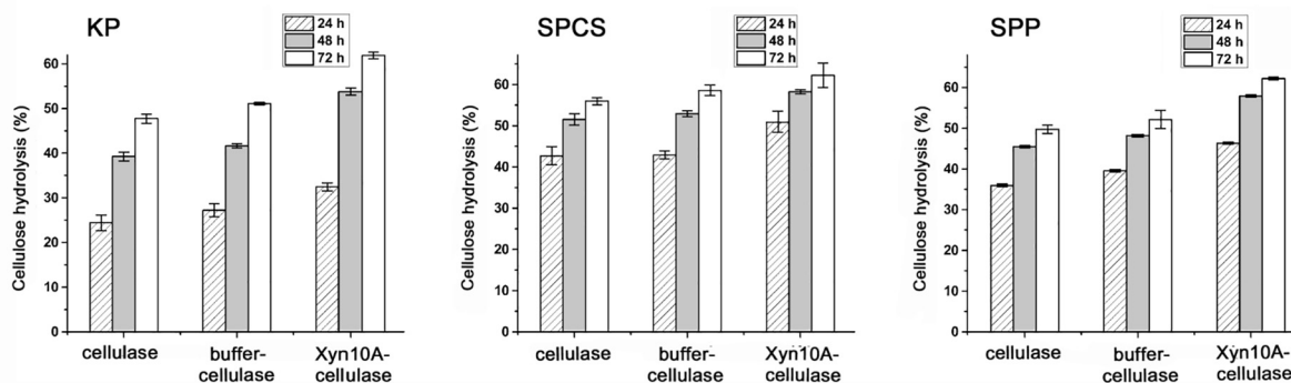
Fig. 2. The extent of cellulose hydrolysis of Kraft pulp (KP), steam pretreated poplar (SPP) and steam pretreated corn stover (SPCS) at 10% solid loading after 24 h, 48 h and 72 h. buffer, substrate was incubated at 85 °C for 3 h without xylanase addition; Xyn10A, hydrolysis in the presence of Xyn10A of 1st stage at 85 °C for 3 h; cellulase, substrate was incubated at 50 °C for 3 h without the addition of xylanase. The statistical analysis showed that the differences (between different hydrolysis time, various substrates, and substrates with/without thermostable xylanase treatment) were all statistically significant (two way ANOVA, p < 0.05 ).
