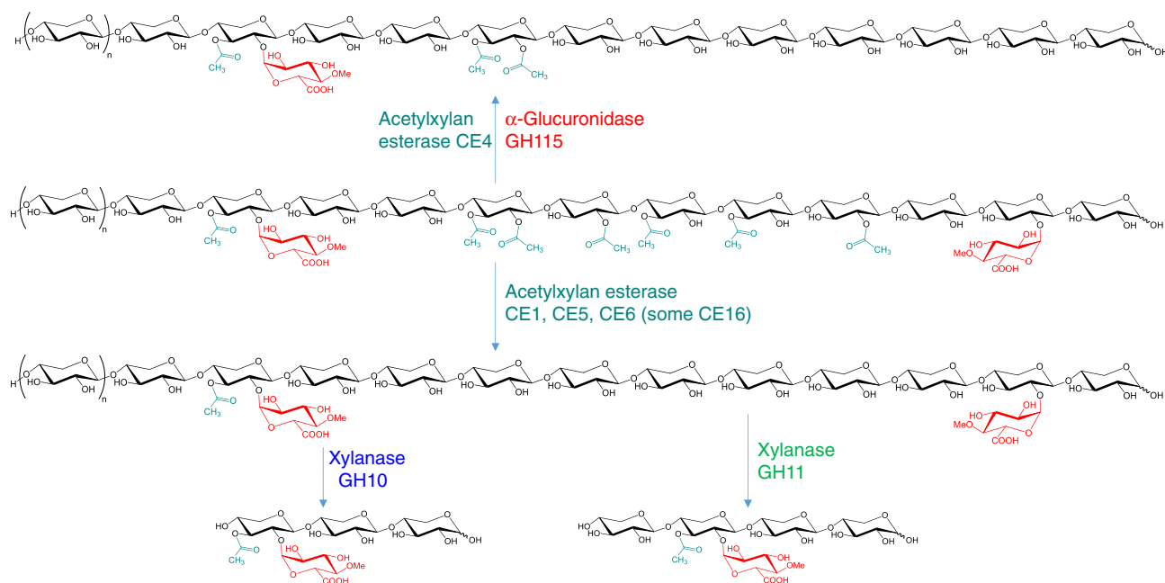
Fig. 3. Scheme of deacetylation of acetylglucuronoxylan (the second chain from the top) by acetylxyylan esterases of CE families 1, 4, 5 and 6 and subsequent degradation by GH10 and GH11 xylanases. Acetylxyylan esterases do not attack the 3- O -acetyl group on Xylp residue substituted with MeGlcA. Doubly acetylated Xylp residues do not serve as substrate for CE4 acetylxyylan esterases. Xylanases of GH families 10 and 11 generate the same aldouronic acids as from deacetylated xylan (Fig. 1; MeGlcA 3 Xyl 3 and MeGlcA 3 Xyl 4 , respectively), but also those which are 3- O -acetylated on Xylp residue substituted with MeGlcA (formulas on the bottom).
