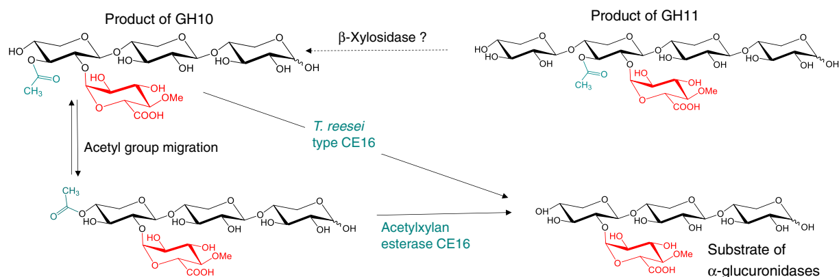
Fig. 4. Degradation pathway of acetylated aldouronic acids generated from acetylglucuronoxylan by GH10 and GH11 xylanases (Fig. 3). The 3- O -acetylated aldotetrauronic acid (Ac 3 MeGlcA 3 Xyl 3 ) can be deacetylated directly by some CE16 deacetylases, e.g. by CE16 from Trichoderma reesei . Alternatively, it can be deesterified by CE16 enzymes in the form of its isomer formed by acetyl group migration to position 4. It remains to be established whether the acetylated aldopentauronic acid formed by GH11 xylanases (Ac 3 MeGlcA 3 Xyl 4 ) does serve as a substrate for \beta -xylosidase (question mark).
