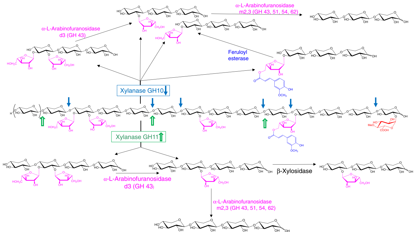
Fig. 5. Scheme of enzymatic breakdown of alkali extracted arabinoglucuronoxylan by xylanases of GH families 10 and 11. Only arabinosylated fragments are shown. Their hydrolysis to monosaccharides requires action of two types of \alpha -L-arabinofuranosidases and \beta -xylosidase. The \alpha -L-arabinofuranosidases are typically active either on 2- or 3-monoarabinosylated Xylp residues (m2,3 type enzymes; GH43, GH51, GH54 and GH62 families) or on doubly arabinosylated Xylp residues (d3 type enzymes; some GH43 members and one GH51 member) from which they liberate solely Araf from position 3.
