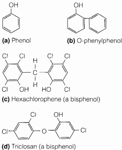
FIGURE 7.7 The structure of phenolics and bisphenols.
