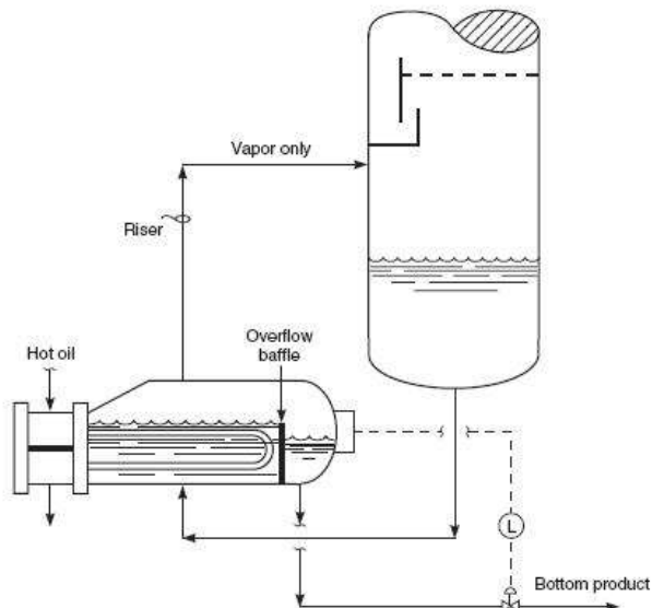
FIGURE 7.7 Kettle reboiler.
